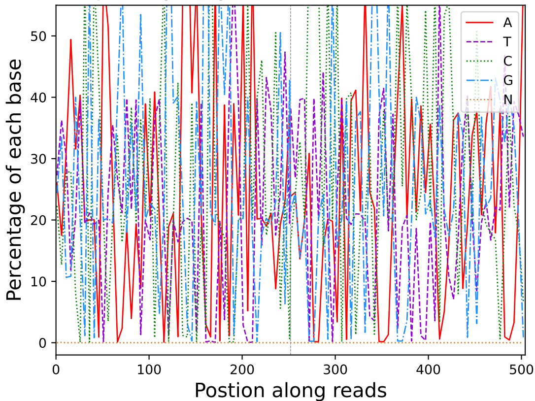
Base percentage along reads (R10715)
